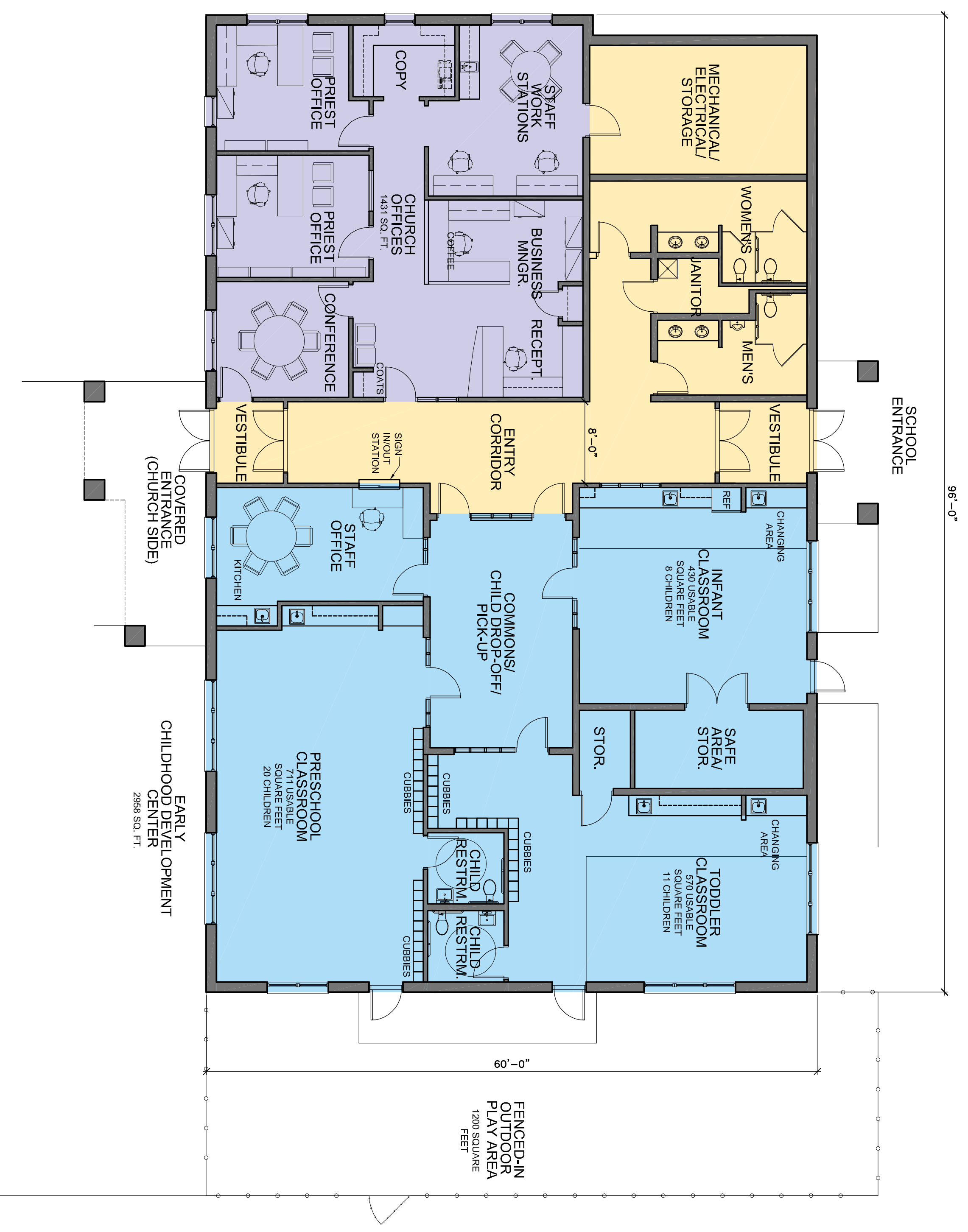
PROPOSED FLOOR PLAN SCALE: 1/8" = 1'-0" 3/16" SQ. FT.
